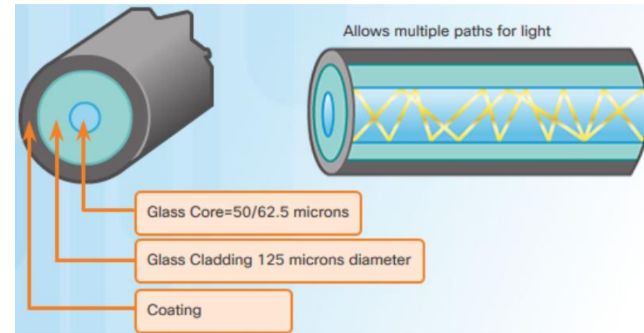
Multimode Fiber
