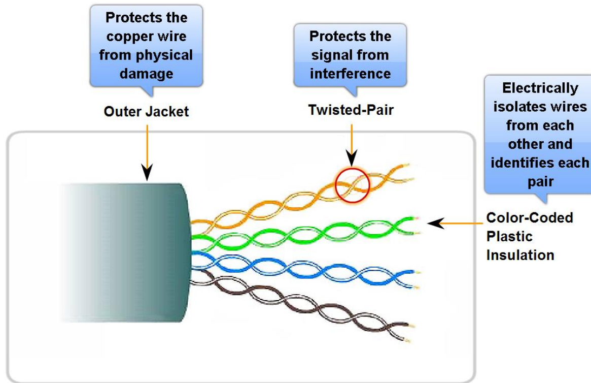
Unshielded Twisted-Pair (UTP) Cable
