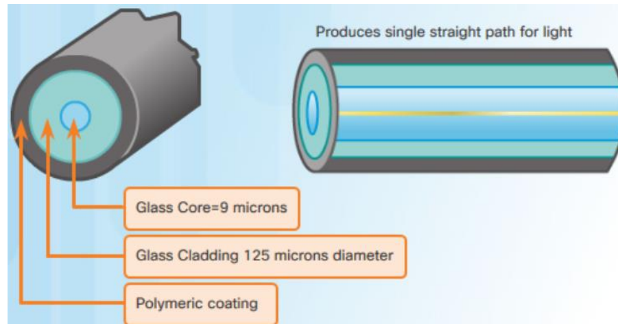
Single-Mode Fiber
